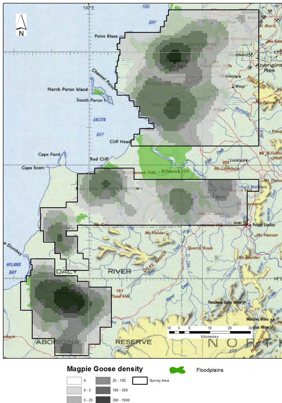
Figure 5a: Magpie Goose density across the Moyle River floodplain to Finniss River floodplain survey area (number per sq. km).
